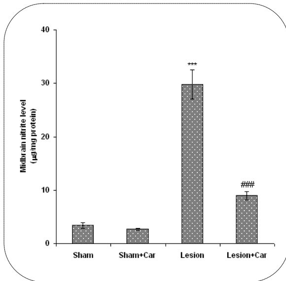
Figure 2. Nitrite content in midbrain homogenate from different groups. Animals were pretreated with carvacrol at a dose of 10 mg/kg before intrastriatal 6-OHDA injection (left side). ***p<0.001 (vs. sham); ###p<0.001 (vs. lesion). (means±SEM).
