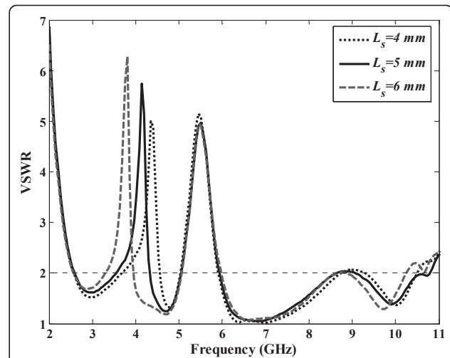
Figure 3 Effect of parameter L_s of T-shaped stub on the antenna's band-notching characteristic.
