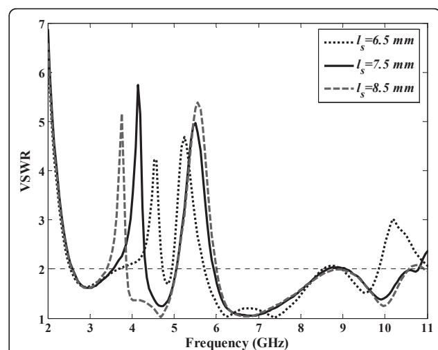
Figure 4 Effect of parameter l_s of T-shaped stub on the band-notched characteristics.
