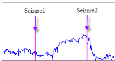
Figure 1. Increase of mean HRV in pre-ictal phase.
