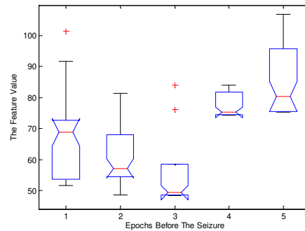
Figure 2. Mean HRV respectively from left to right for 180-90min, 90-30min, 30-10min, 10-5min, and 5 min before the seizure
